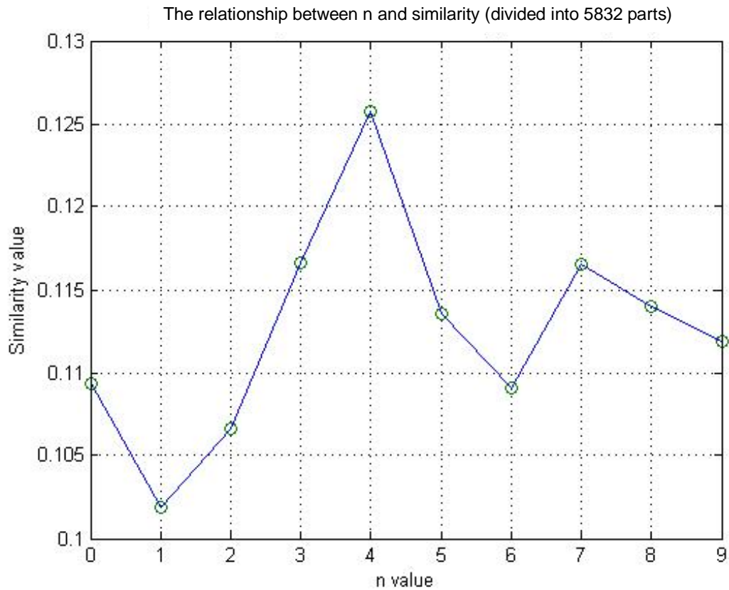
Figure 6. The trend of similarities for differential length of linker when the number of portions is 18^3 .
