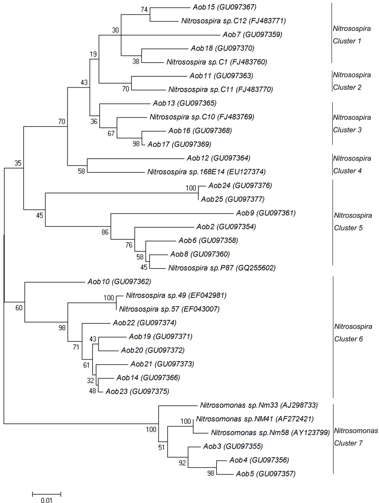
Figure 4. Phylogenetic analyses of ammonia monooxygenase genes recovered from DGGE bands of paddy soil under different management. The bar indicates an estimated 1% sequence divergence. Bootstrap values are given for 1000 replicate trees.
