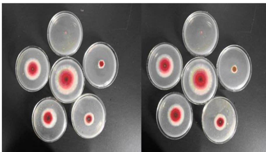
Figure 1. Inhibitory activity of xa202 and xt208 against mycelial growth of G. zeae . The left-hand chart and the right-hand chart represent respectively the inhibitory picture of xa202 and xt208 (concentration are 25.0, 12.5, 6.25, 3.13, 1.56 µg/ml). The concentration in the clockwise direction at the chart arranged from large to small order.
