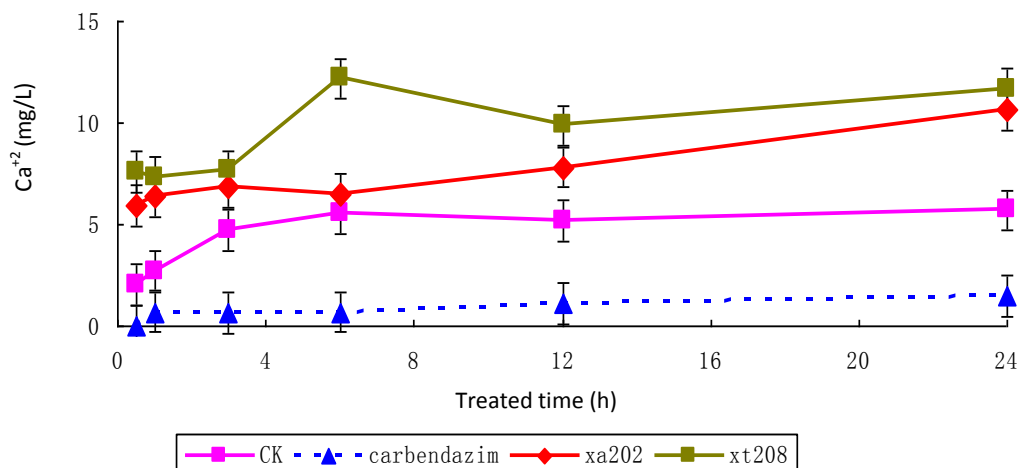
Figure 3. Content change of the Ca 2+ in the mycelium of Gibberella zeae .
