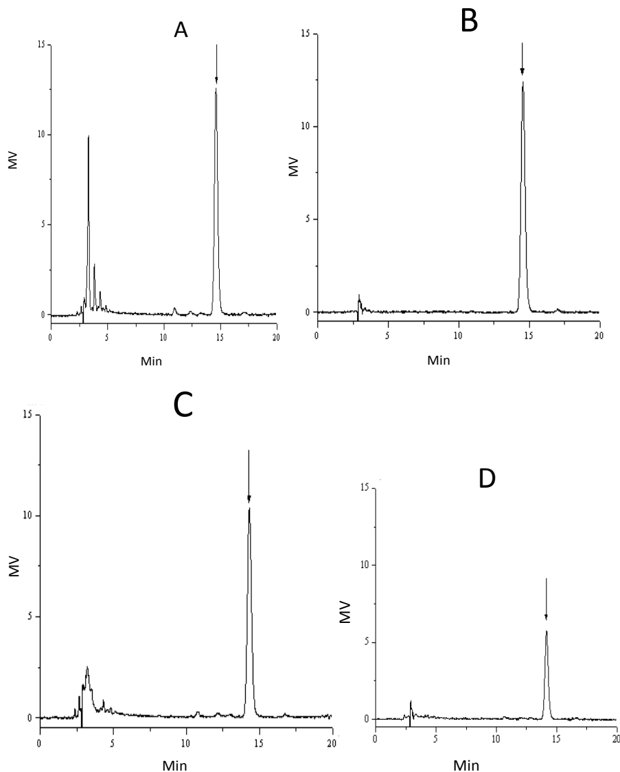
Figure 5. Chromatogram of ergosterol in mycelium with the different conditions. A: blank control ; B: carbendazim ; C : xa202 ; D : xt208.
