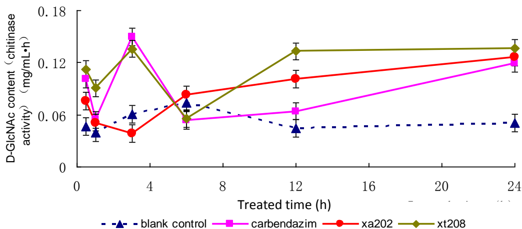
Figure 2. Change of the mycelial chitinase activity in the mycelium of G. zeae .
