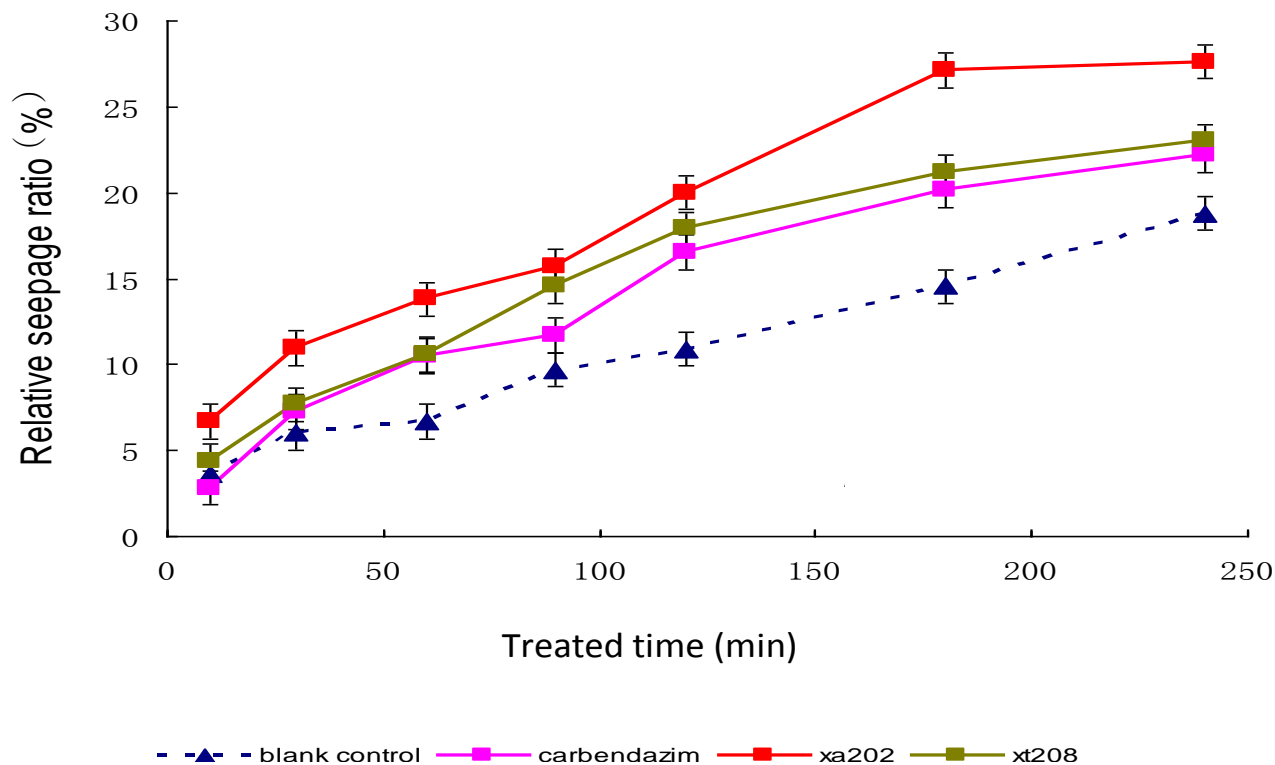
Figure 4. Effect of compounds xa202 and xt208 on membrane permeability of G. zeae .
