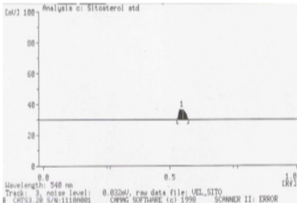
Figure 3. HPTLC Chromatogram of beta sitosterol standard
