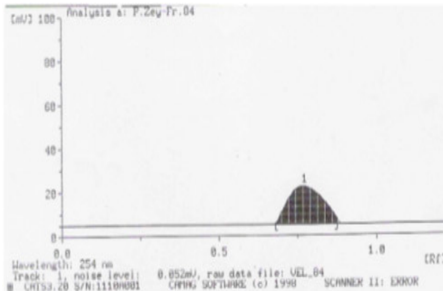
Figure 4. HPTLC Chromatogram of guggultetrol-18-ferrulate
