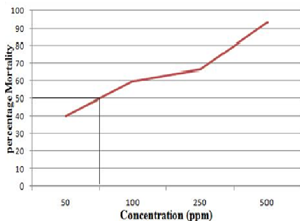
Graph 3. Cytotoxicity of Guggultetrol-18-ferrulate (Graph for LC50).
