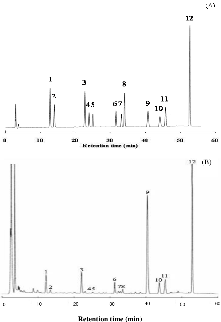
Figure 3. HPLC profile of isoflavone of standard (A) and defatted soybean fermented by Bifidobacterium longum BCRC 14661 at 37°C for 48 h (B). 1, Daidzin (12.80 min); 2, Glystin (14.07 min); 3, Genistin (22.86 min); 4, Malonyldaidzin (24.08 min); 5, Malonylglycitin (25.15 min); 6, Acetyldaidzin (31.84 min); 7, Acetylglystin (33.39 min); 8, Malonylgenistin (34.32 min); 9, Daidzein (41.10 min); 10, Glycitein (44.51 min); 11, Acetylgenistin (46.11 min); 12, Genistein (53.10 min).
