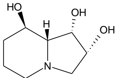
Figure 1. Structure of swainsonine.
