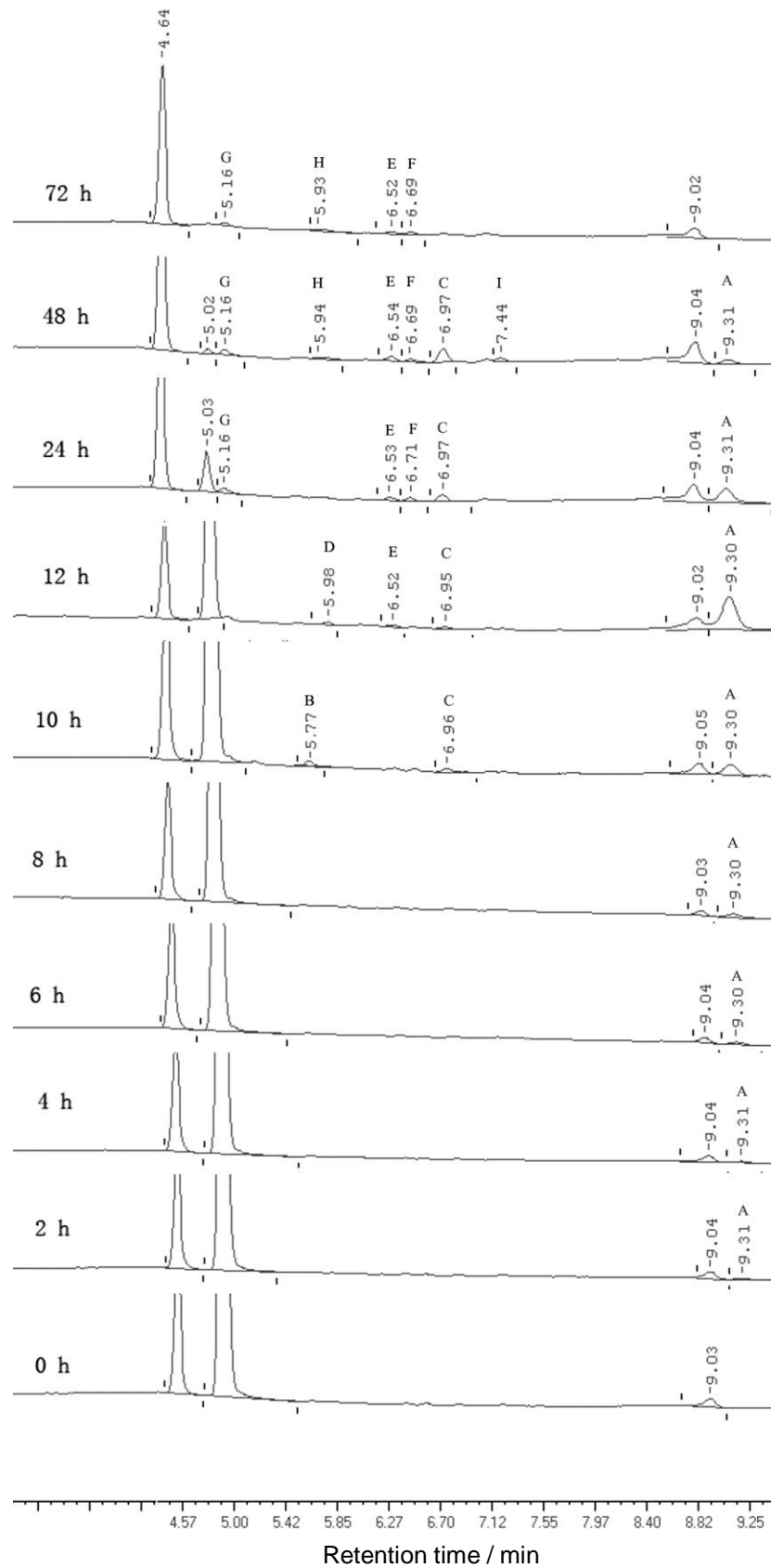
Figure 4. The gas chromatography of 1 g -1 SW degradation by the mixture of 5 types of transformants in 72 h.
