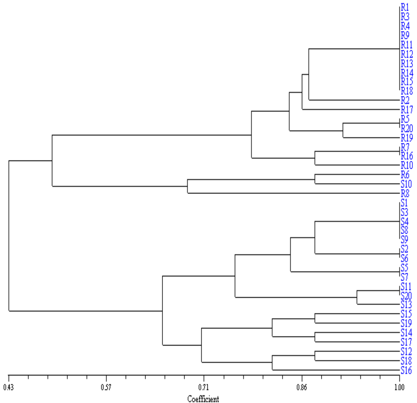
Figure 3. Phylogenetic relationship of the 40 cowpea lines constructed using four microsatellite polymorphisms.
