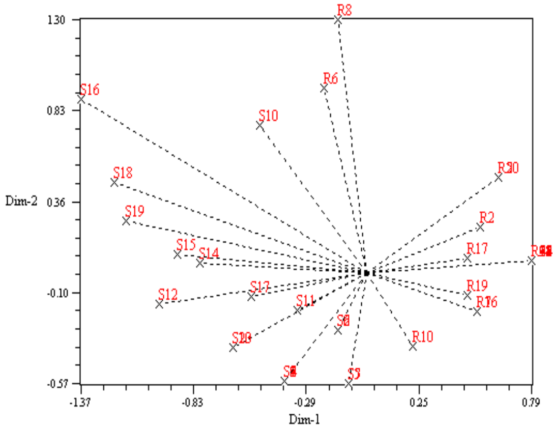
Figure 4. Two-dimension principle coordinates analysis of the 40 cowpea lines.
