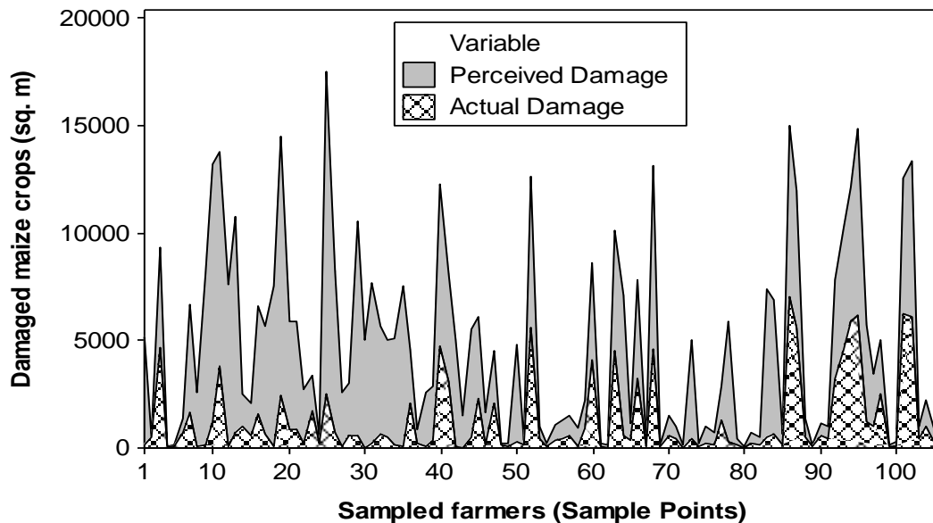
Figure 2. Comparison between the perceived and actual damage by wildlife in sample points for maize crop in the Luangwa Valley, Zambia, 2006/7 and 2007/8.
