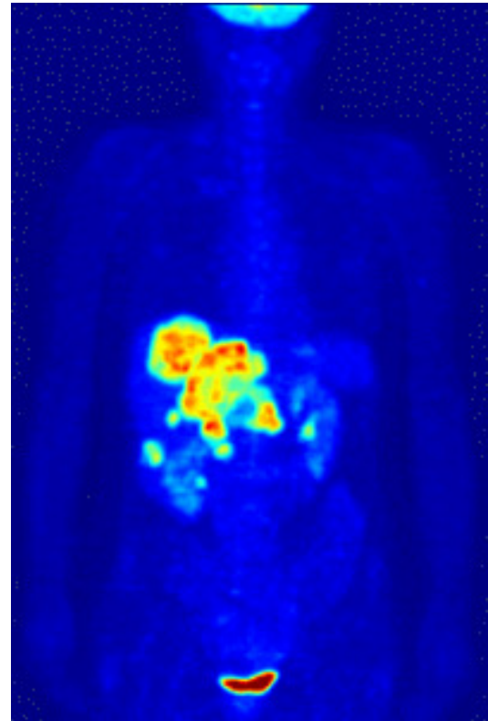
Figure 3. Fluorine 18 .
