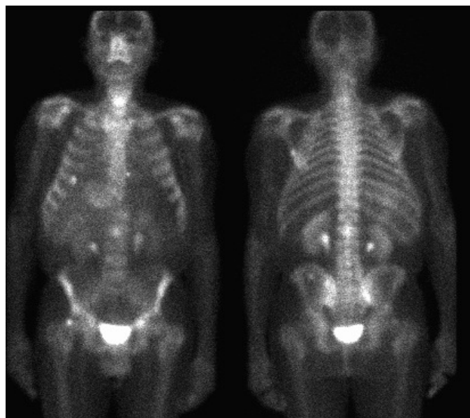
Figure 2. Tc-99m MDP.
