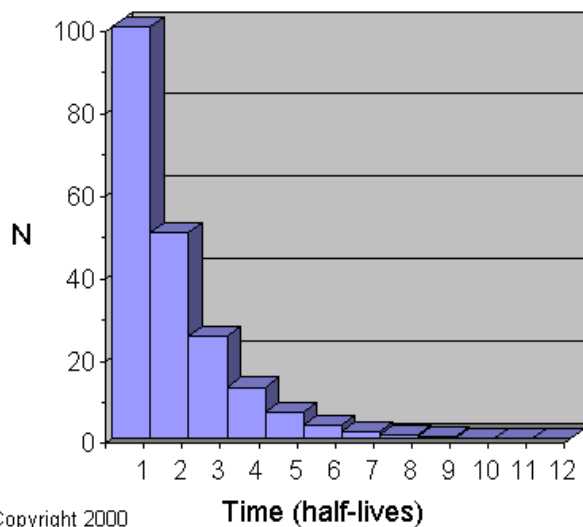
Figure 1. Tc-99m MDP
