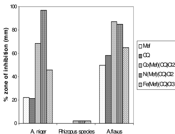
Figure 2. Inhibitory activity of the ligands and metal complexes against Aspergillus niger , Rhizopus species , and Aspergillus flavus .
