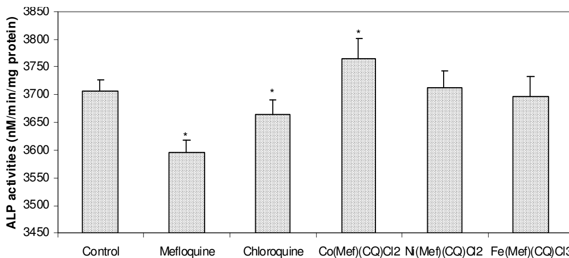
Figure 4. Effect of administration of ligands and metal complexes on the activities of alkaline phosphatase of rat kidney. *Significantly different from the control ( p < 0.05 ).
