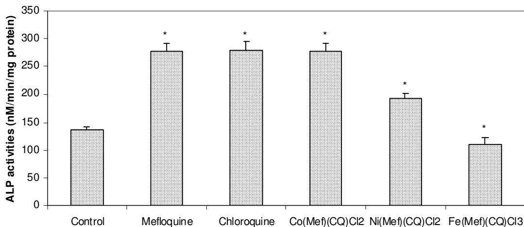
Figure 5. Effect of administration of ligands and metal complexes on the activities of alkaline phosphatase of rat liver. *Significantly different from the control ( p < 0.05 ).
