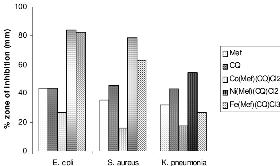
Figure 1. Inhibitory activity of the ligands and metal complexes against Escherichia coli , Staphylococcus aureus and Klebsiella pneumonia .
