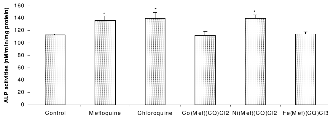
Figure 3. Effect of administration of ligands and metal complexes on the activities of alkaline phosphatase of rat serum. *Significantly different from the control ( p < 0.05 ).
