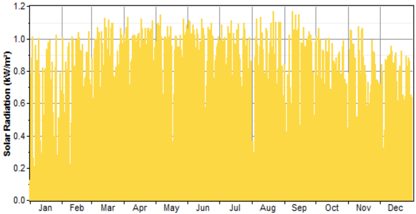
Figure 4a. Annual evolution of solar irradianations. Source: Simulation by HOMER
