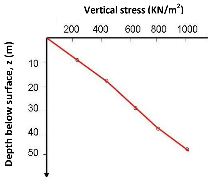
Figure 5. The relationship between vertical stress and depth above the tunnel.
