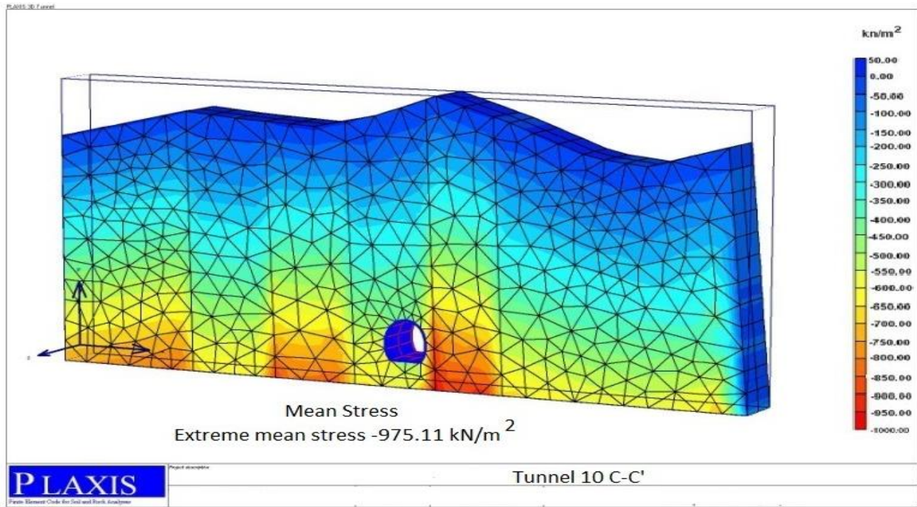
Figure 6. The stress distribution surrounding the tunnel in a cross section.
