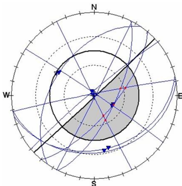
Figure 9. Analysis stability of rock blocks in tunnel wall.
