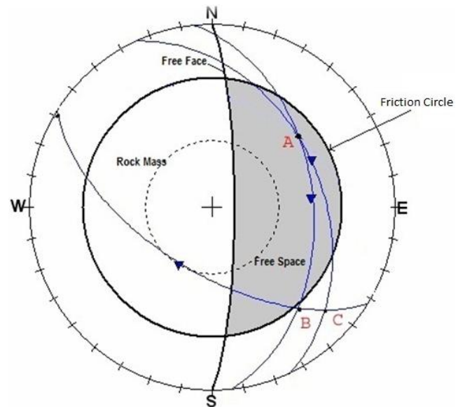
Figure 3. The relationship of planes with friction circle in free face of rock mass.
