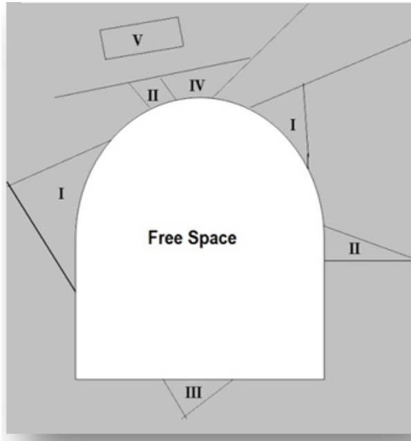
Figure 1. Type of blocks around the excavation section.
