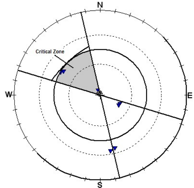
Figure 10. Analysis stability of rock blocks in tunnel roof.
