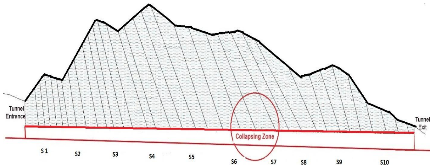
Figure 4. The tunnel with vertical bedding in sandstone mass.
