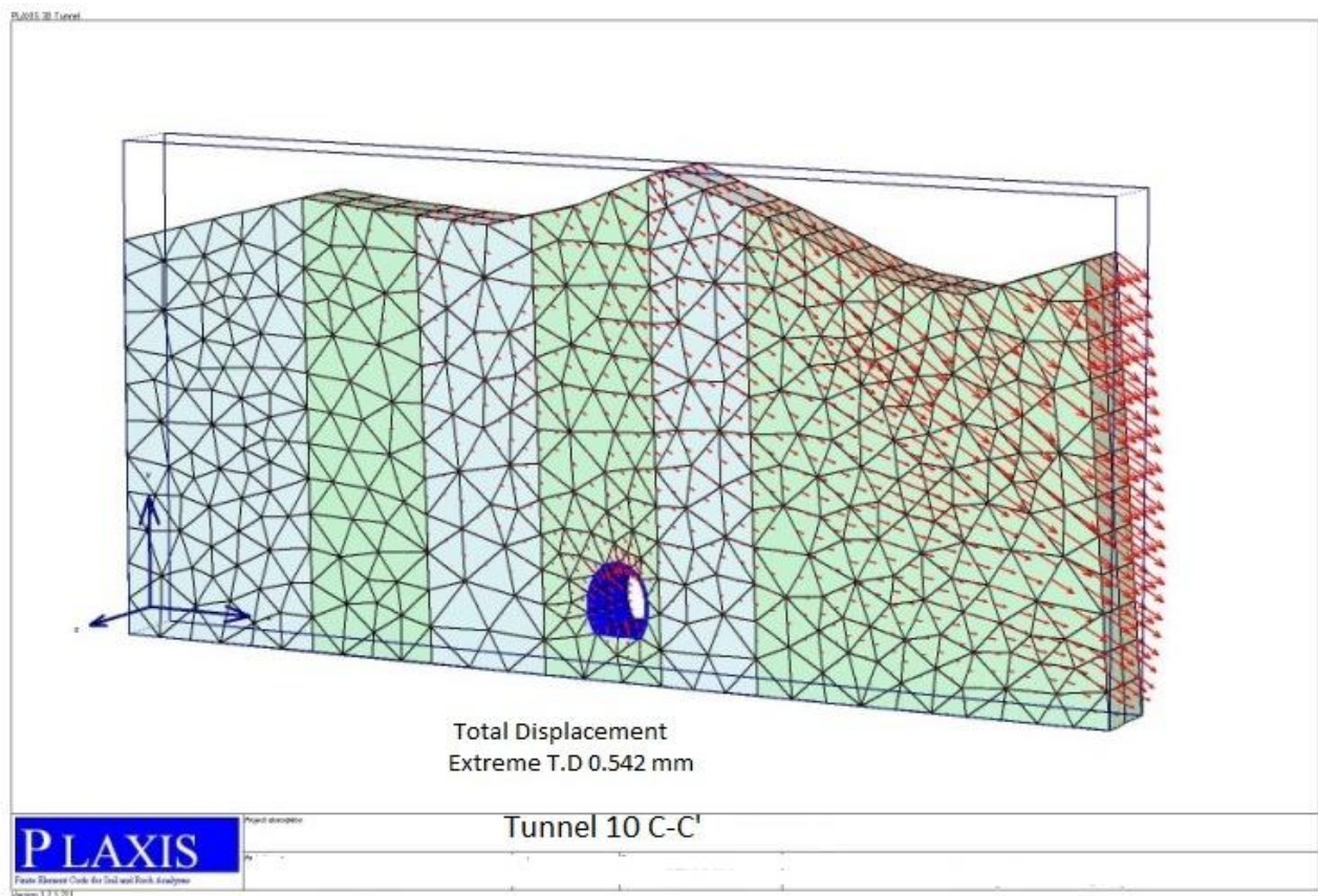
Figure 7. Total displacement of rock mass around the tunnel.
