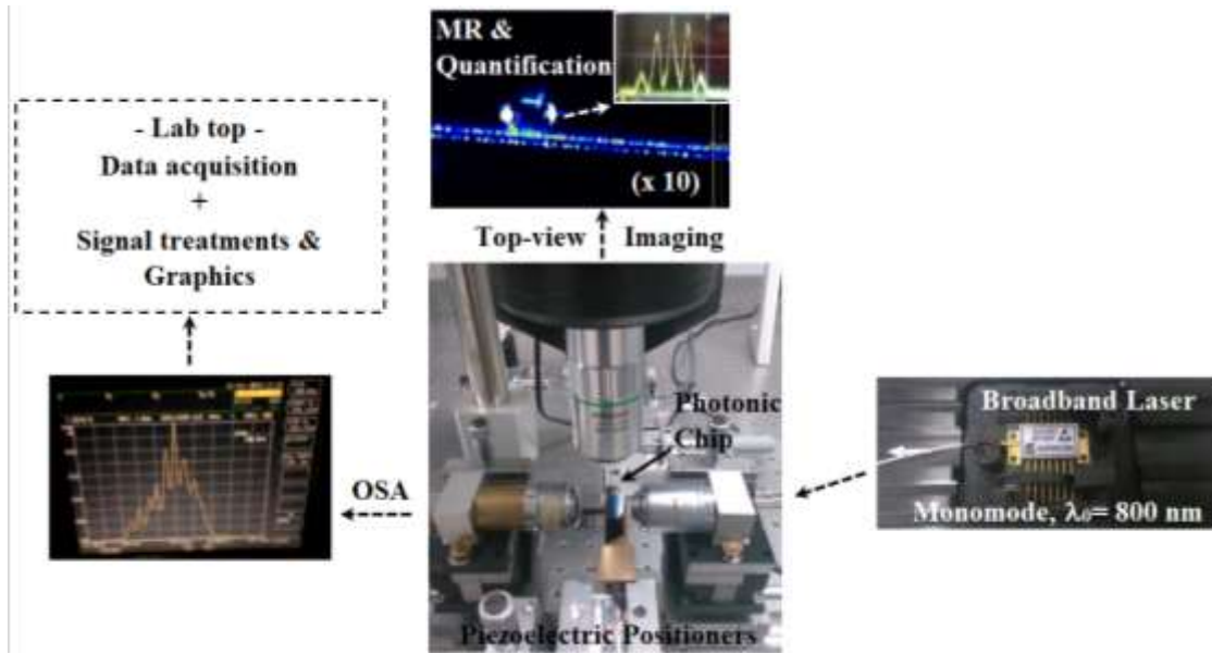
Figure 6. Principles and photographs of various part of the experimental setup. A broadband laser source is used to excite the slot MRs structures ( \lambda_{0-center} = 800 nm). The quantified light is then sent to an Optical Spectrum Analyzer (OSA). The surface of the chip is highlighted due to imaging from above. A specific software controls the whole set of data acquisitions together with the signal processing of spectra in real time.
