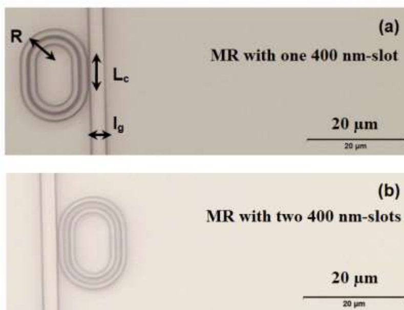
Figure 5. Upper-view (optical imaging: magnification \times 50 ) of photonic micro-resonators with inscribed nano-slots featuring a 400 nm fixed width. Such racetrack micro-resonators (MRs) present a radius of curvature R = 5 \mu\text{m} and a 5 \mu\text{m} coupling length, L_c : Both waveguides have a same width l_g = 3 \mu\text{m} . (a) MR with one slot, (b) MR with two slots. In such MR configurations, perimeter L_{\text{geo}} = 41.5 \mu\text{m} .
