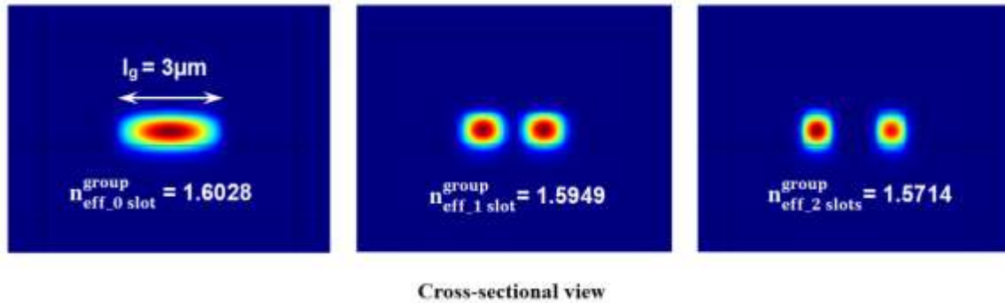
Figure 3. COMSOL Multiphysics: Simulations I 2D ; COMSOL simulations: calculations of the eigenvectors (spatial distributions of the single mode quasi-TE) plus the eigenvalues as the so-called effective group indices n_{eff}^{group} associated to each family of waveguides with respectively; 0, 1 and 2 inscribed nano-slots. With such a cyclic and geometric resonant principle, effective indices are inversely proportional to the above-mentioned FSR measurements ( n_{eff}^{group} \propto 1/FSR^{group} , see equation (3)).
