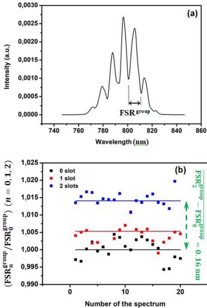
Figure 7. (a) Example of a spectrum transduced by a MR structure. Free Spectral Range ( FSR_{group} ) represents the pseudo-period of the spectrum signal. (b) Calculation of FSR_n^{group} ( n = 0, 1 and 2 slots) normalized to the average of FSR_0^{group} . Such averages are determined on a 20 experimental spectra statistic.
