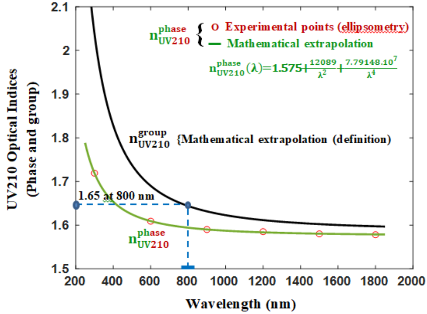
Figure 1. Dispersion curves of the UV210 material: optical phase index n_{UV210}^{phase} of the material measured by ellipsometry plus mathematical extrapolation; the result of Cauchy's law is then estimated as n_{UV210}^{phase}(\lambda) = 1.575 + \frac{12089}{\lambda^2} + \frac{7.79148 \cdot 10^7}{\lambda^4} . The extrapolation of the group index of the UV210 material n_{UV210}^{group} is obtained by the classical optical definition that links n_{UV210}^{phase}(\lambda) with a gradient.
