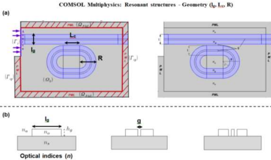
Figure 2. COMSOL Multiphysics: Geometry of the resonant structures. (a) Upper-view of the resonant structures. Such racetrack micro-resonators (MRs) present a radius of curvature R = 5 \mu\text{m} and a 5 \mu\text{m} coupling length, L_c : Both waveguides have a same width l_g = 3 \mu\text{m} (MR with one slot in such example). Beyond the structure, \Omega_{\text{PML}} represents an area called ‘Perfectly Matched Layer’ avoiding untoward reflections for simulations. The indices of the structure for the study in propagation and spectral resonances will be fixed to the values of the effective indices of the structures; (b) Schematic diagram of the cross-sectional view of the three family waveguides structures respectively made of a rib with no slot and ribs with 1 and 2_ slots nano-inscribed. At a wavelength of \lambda_{00} = 800 \text{ nm} , optical indices of the materials are fixed for the simulations at n_a = 1.00 (air, upper-cladding), n_o = 1.65 (group index of the polymer UV210, core waveguide) and n_s = 1.45 (Silica, lower-cladding). The other parameters describe the geometric dimensions with: l_g = 3 \mu\text{m} as the width of the global rib waveguide, its thickness h_g = 1 \mu\text{m} , and g = 400 \text{ nm} the common width of each nano-slot.
