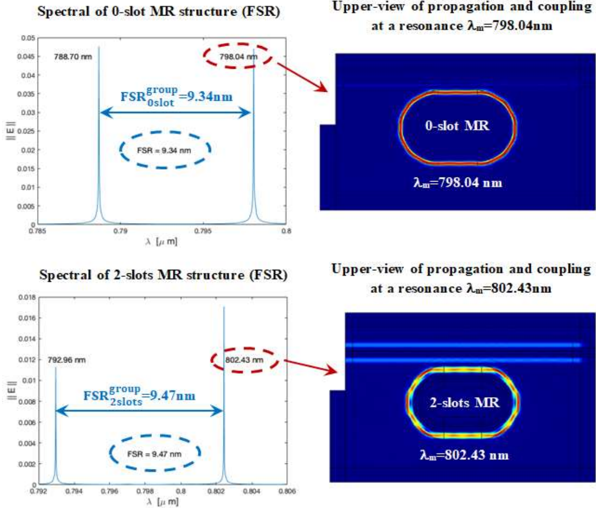
Figure 4. COMSOL Multiphysics: Simulations II 3D ; geometry and parameters previously defined in Figure 2 (a). COMSOL simulations: determination of each spectral resonance (entailing FSR^{group} values) for the 0-slot and the 2-slot structures so as to evaluate the global ranging effect of mass recessing (nano-gap of air) within the studied structures.
