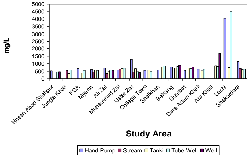
Figure 6. Total solids in water samples.
