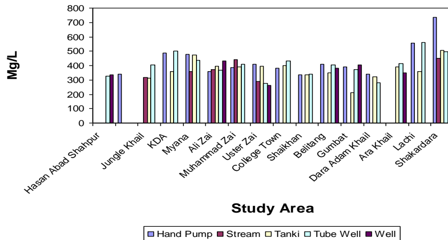
Figure 2. Total alkalinity of water samples.
