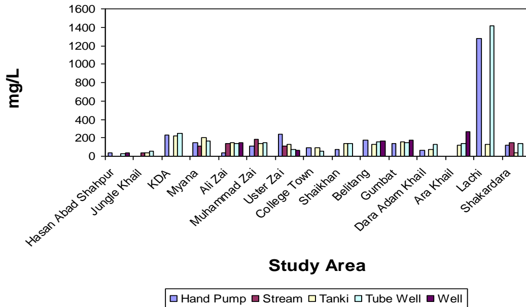
Figure 10. Chloride in water samples.
