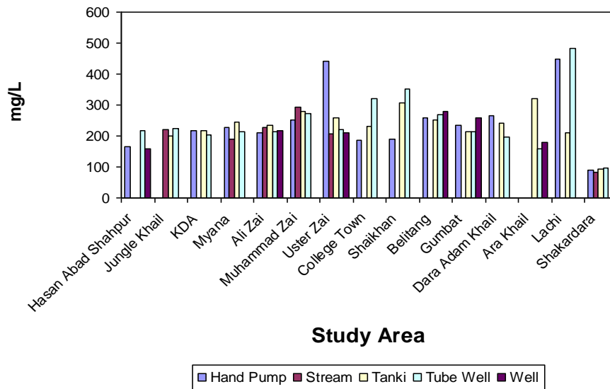
Figure 7. Calcium hardness in water samples.
