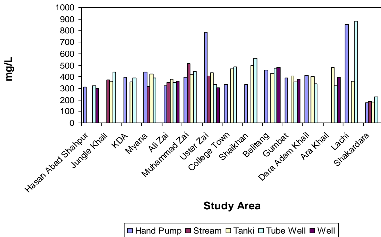
Figure 9. Total Hardness in water samples.
