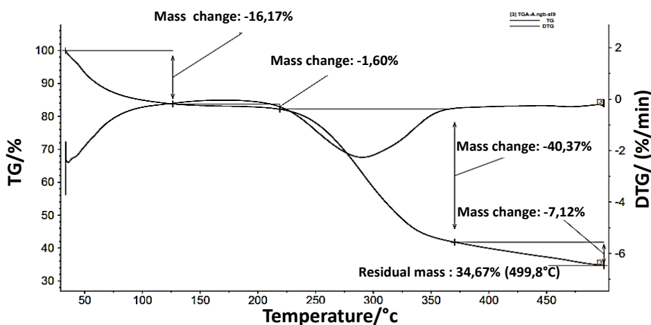
Figure 10. Thermogravimetric analysis of Grewia spp. Biopolymer.
