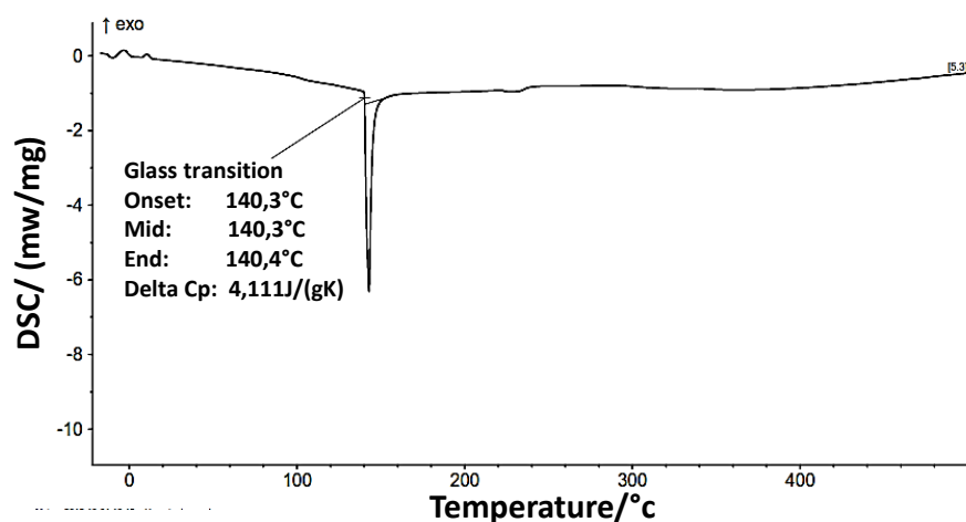
Figure 9. Differential Scanning Calorimetry graph of Grewia spp. biopolymer
