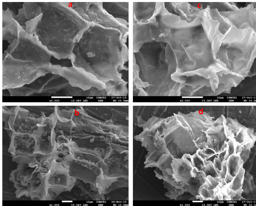
Figure 7. SEM images of Grewia spp. biopolymer before (a, b) and after purification (c, d).
