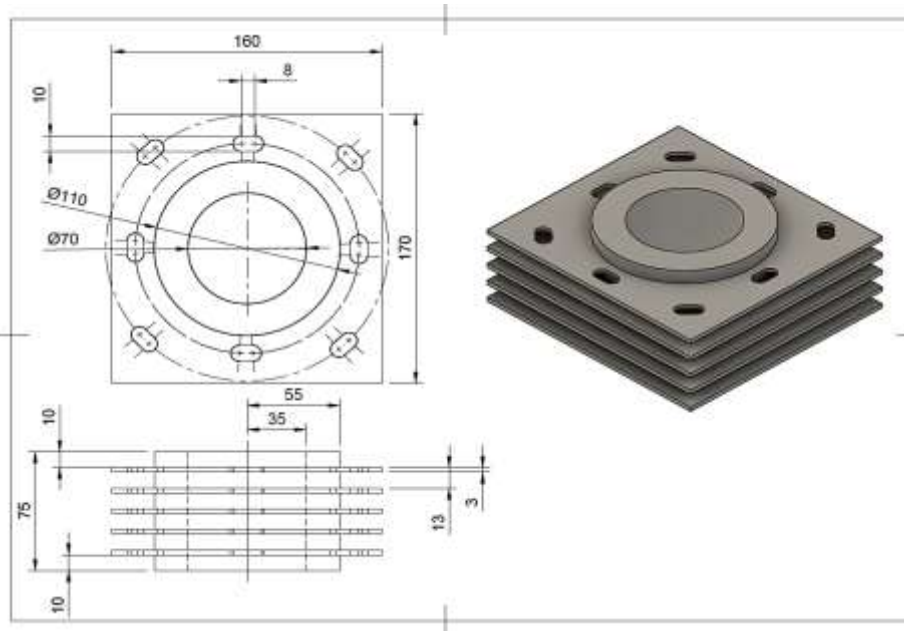
Figure 3. Rectangular fin model of 3 mm thickness with slots.
