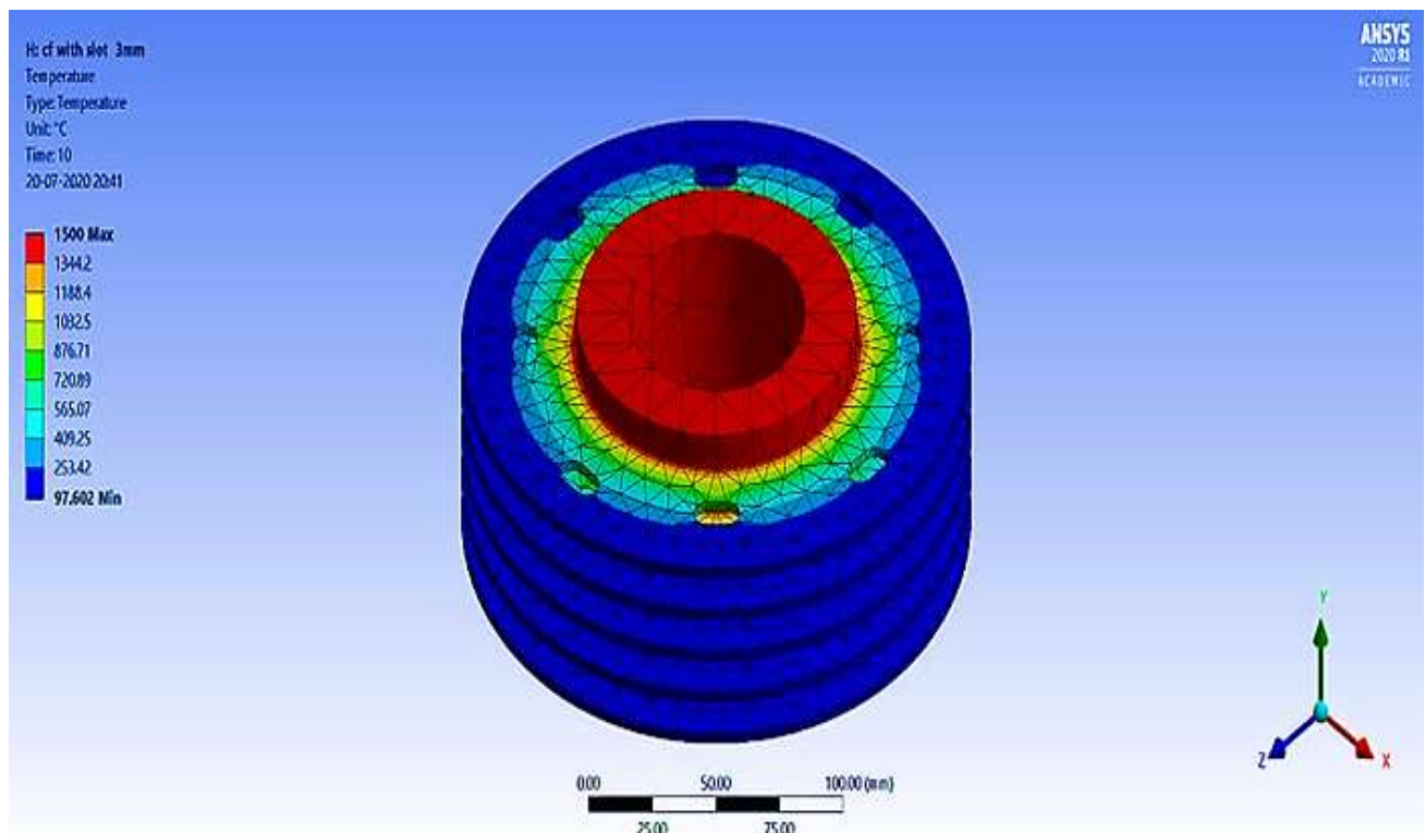
Figure 17. Temperature distribution in Circular fin 3 mm thickness with slot.
