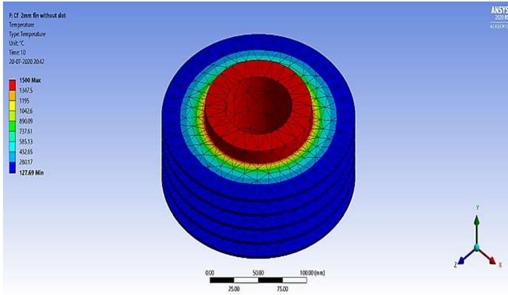
Figure 14. Temperature distribution in Circular fin 2 mm thickness without slot.
