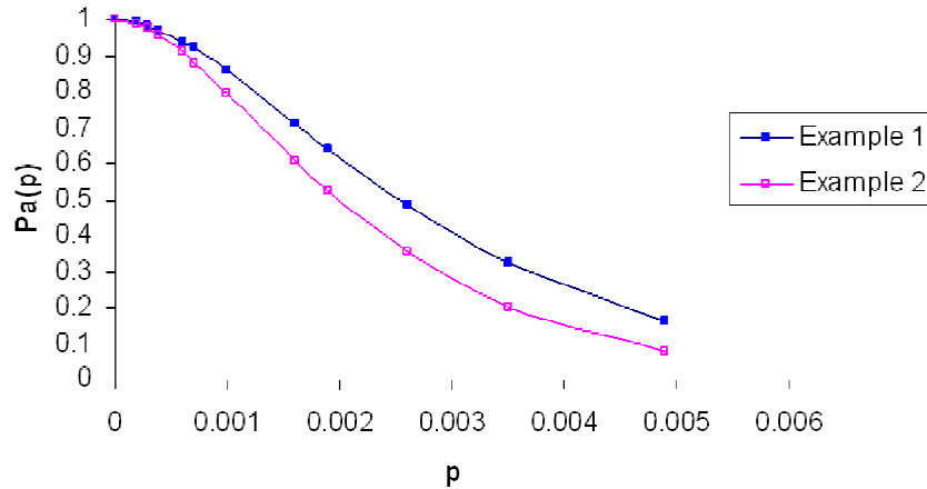
Figure 1. OC curves for the plan n = 667 and i = 2 and n = 850 and i = 3 .
