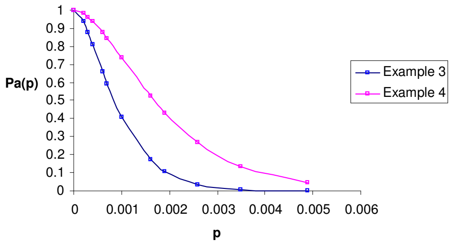
Figure 2. OC curves for the plan n = 2003 and i = 1 and n = 1002 and i = 2 .
