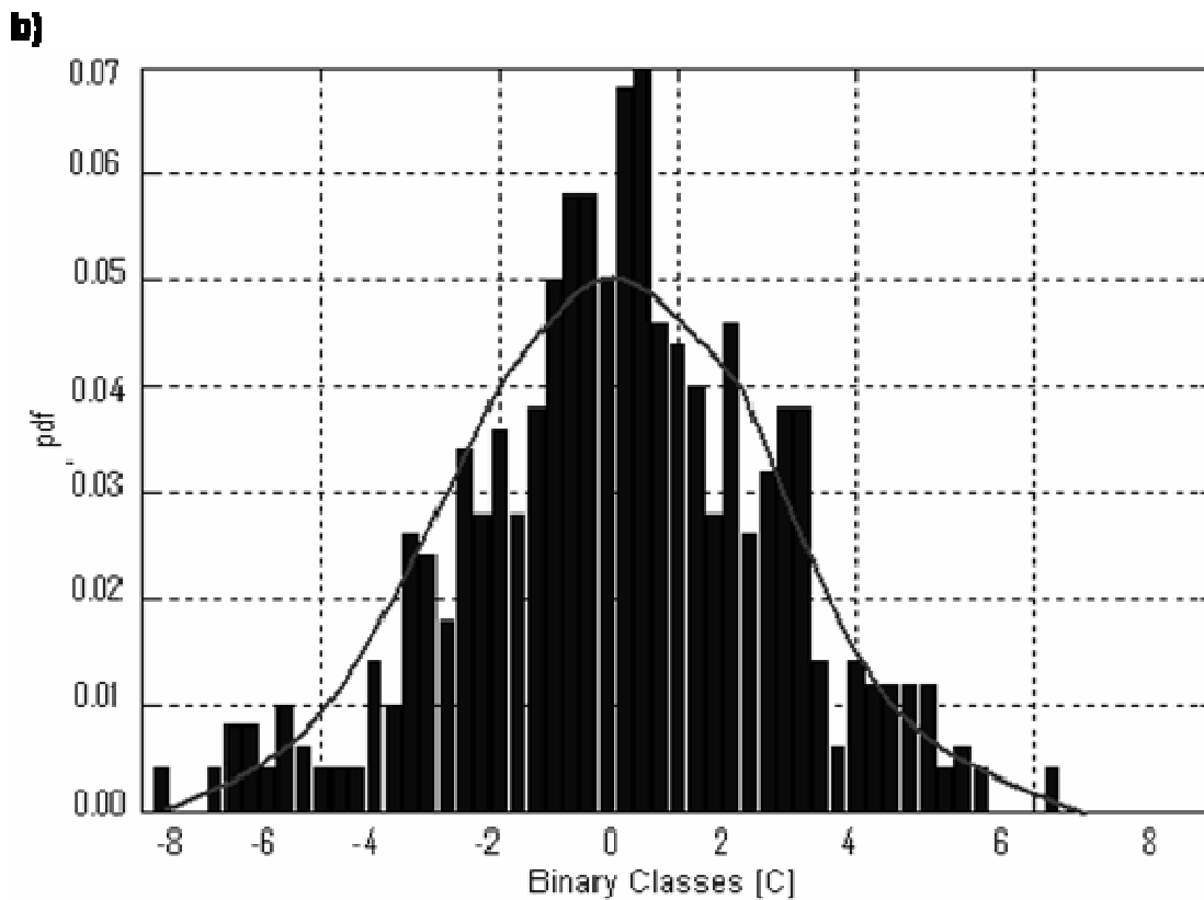
Figure 5b. Histogram and respective Gaussian pdf for random component of \Theta_M ; Data from 2005.
