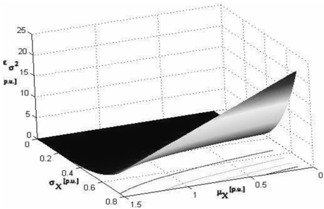
Figure 16a. First order linearisation error \epsilon_\mu .
