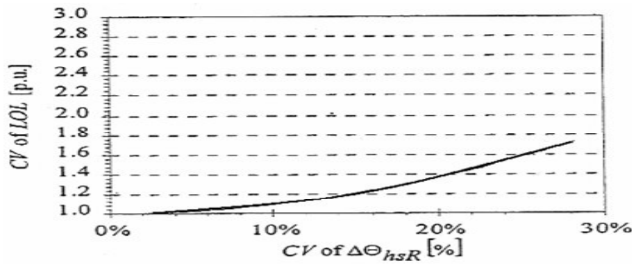
Figure 22b. LOL sensitivity to \Delta\Theta_{hsR} variability.
