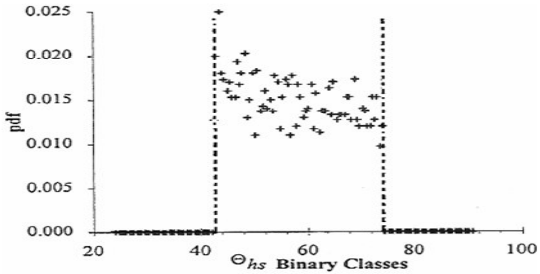
Figure 21a. \Delta\Theta_{hs} pdfs for Normal inputs.
