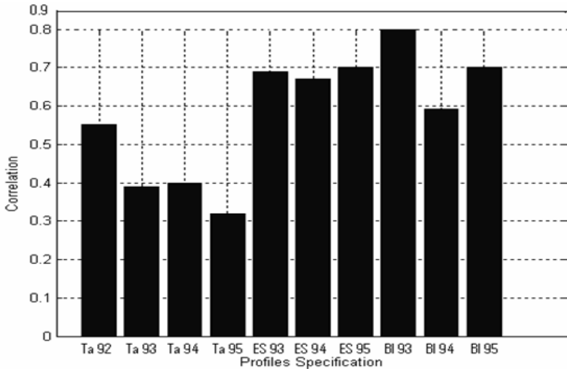
Figure 12. Correlation between random components x_{av\_rand} and x_{am\_rand} .
