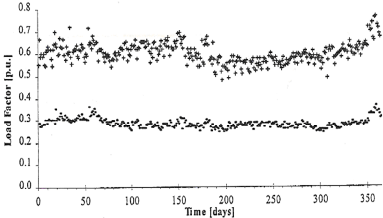
Figure 7. Annual time series representing daily maximal (denoted with +) and minimal (denoted with -) load factor of distribution transformer ESI. Data from 2005.
