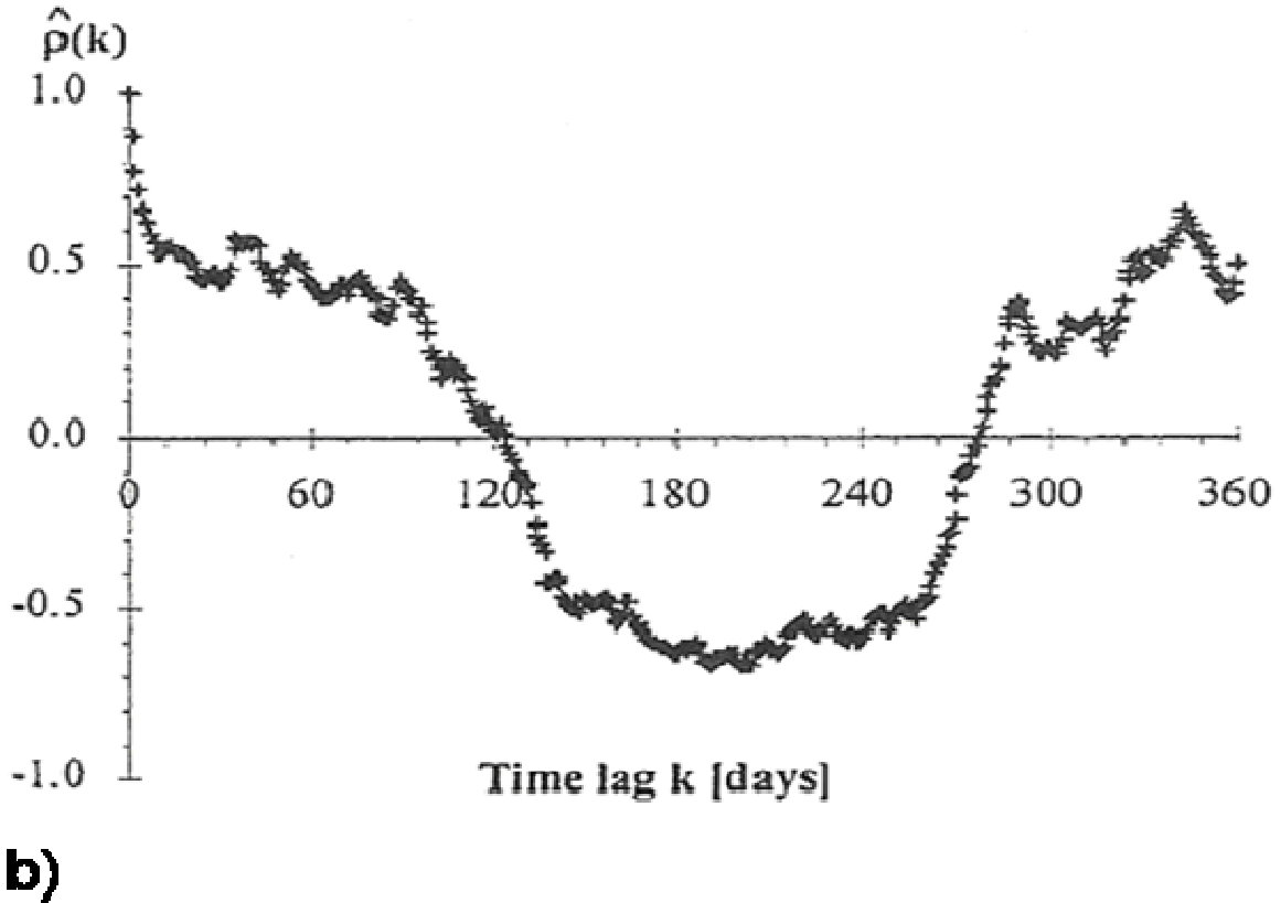
b) Figure 2b. Autocorrelogram of daily maximal ambient temperatures in 2004 and 2005.
