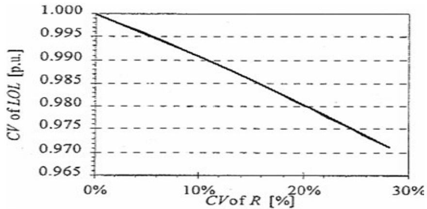
Figure 23. LOL sensitivity to R variability.
