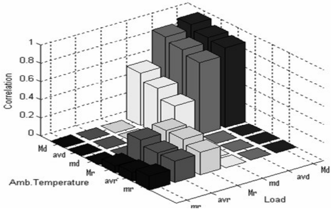
Figure 13. Deterministic and random correlation between ambient temperature and ESI Data from 2004. (Table 6 for ESI transformer).
