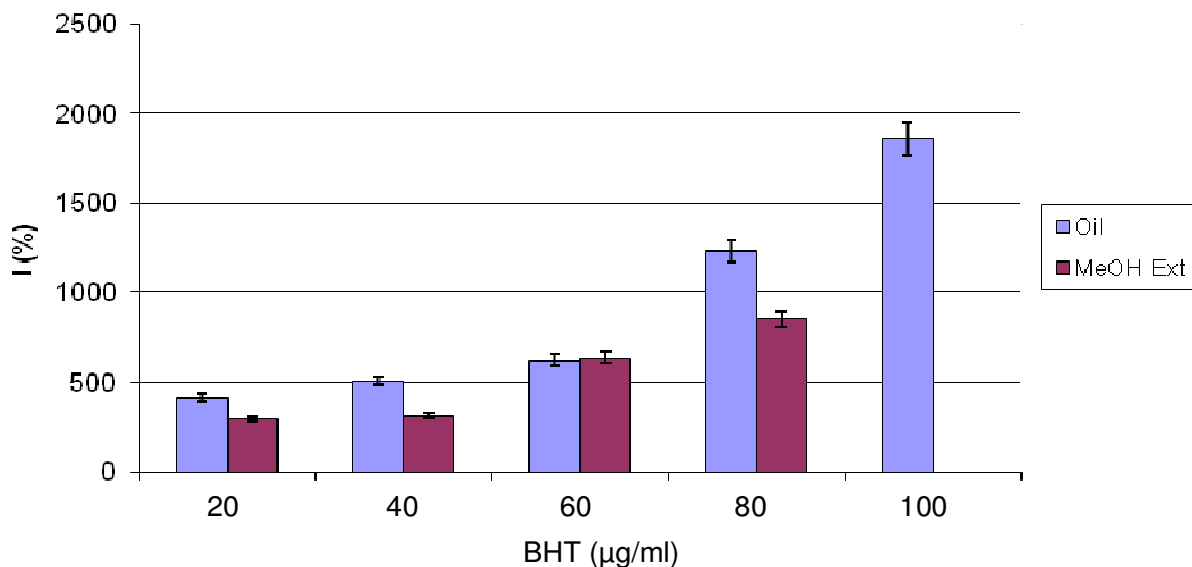
Figure 2. DPPH radical scavenging activity of essential oil and methanol extract of M. Chamomilla . IC 50 of essential oil and methanol extract respectively 4.18 µg/mL and 1.83 µg/ml, I=%DPPH radical scavenging=[(control absorbance- sample absorbance)]/control absorbance] X 100.
