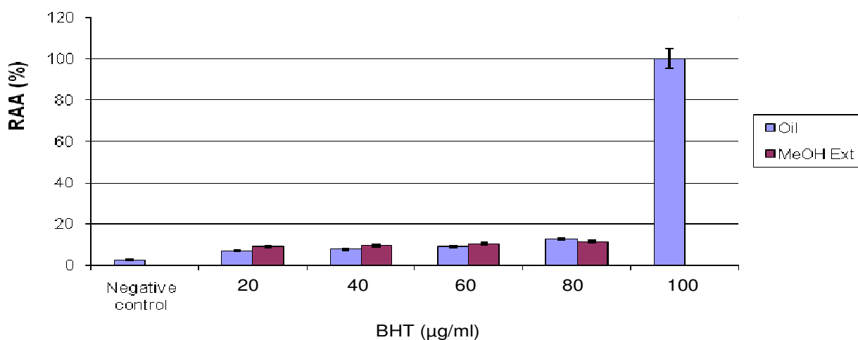
Figure 1. β-carotene bleaching test of M. Chamomilla , essential oil and methanol extract. RAA: Relative Antioxidant Activity= (sample absorbance/BHTabsorbance) X 100, BHT: 2, 6-di-tert-butyl-4-methylphenol or 2, 6-Bis (1, 1-dimethylethyl)-4-methylphenol.
