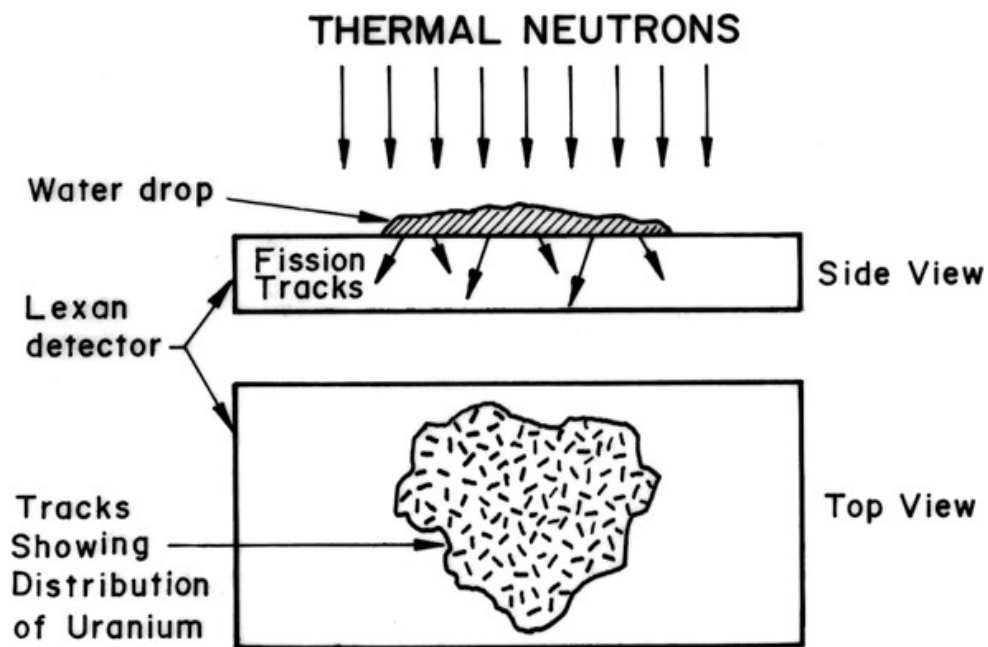
Figure 2. Schematic representation of the Neutron Induced Fission Technique used for uranium determination in drinking water.
