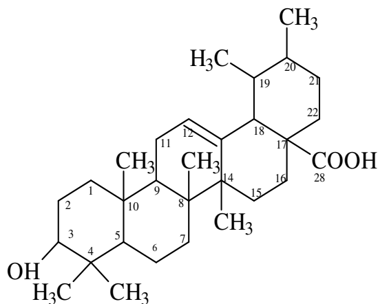
Figure 2. Ursolic Acid. [ 3\beta -hydroxy-urs-12-en-28-oic acid].
