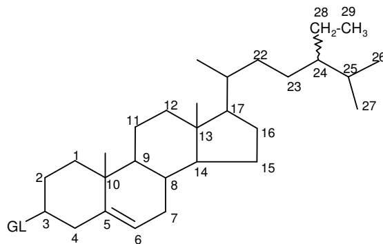
Figure 3. \beta -Sitosterol \beta -D-Glucoside.
