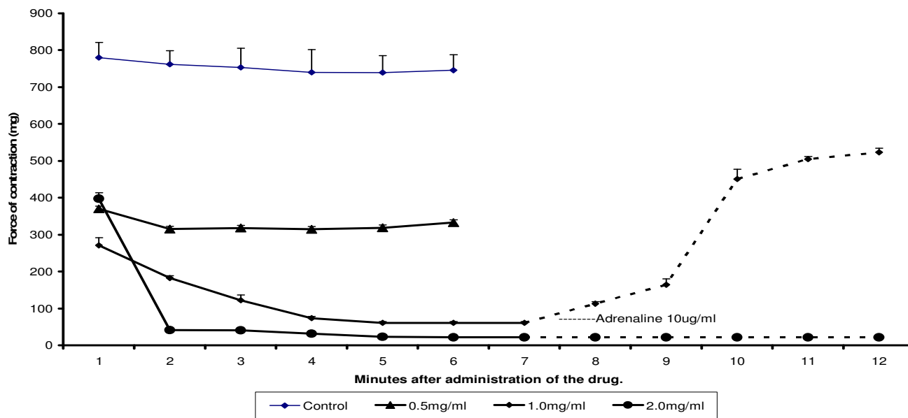
Figure 3. Effect 3, 4-dihydroxybenzaldehyde isolated from the stem bark of M. cecropioides on the force of contractions of isolated rabbit heart. It remarkably reduced the force of contractions of the heart at 1 and 2 mg/ml. The inhibitory effect of 1mg/ml was reversed by Adrenaline 10 \mu g/ml (-----) while the effect of 2mg/ml was irreversible (n = 3).
