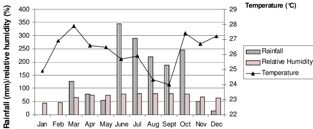
Figure 1b. The chart of rainfall distribution, relative humidity and temperature regime of Akure in 2008. Source: Ondo State Agroclimatological Unit, Ministry of Agriculture and Natural Resources Akure.
