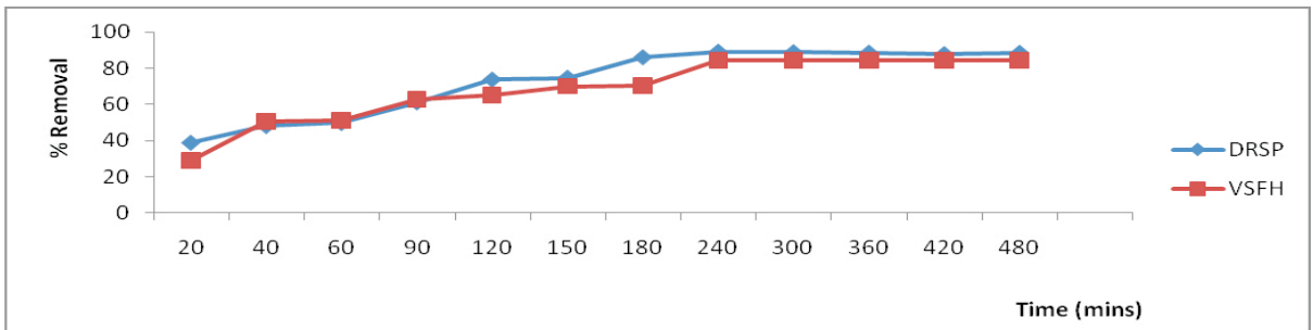
Figure 6. Plots of removal efficiencies against contact time.
